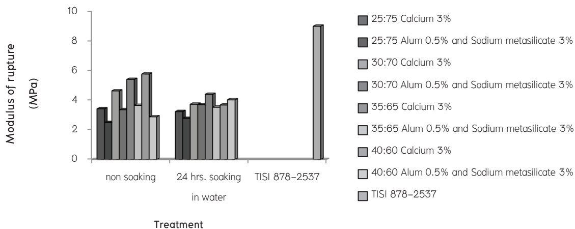
Figure 3. Modulus of rupture of wood cement boards from Azadirachta indica A. Juss.
