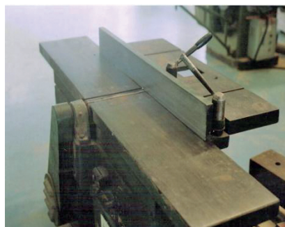
Figure 5 Jointer planer
