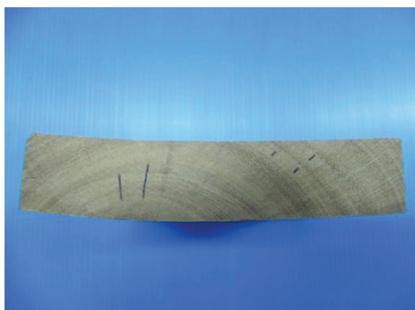
Figure 7. Measuring honeycombing.
