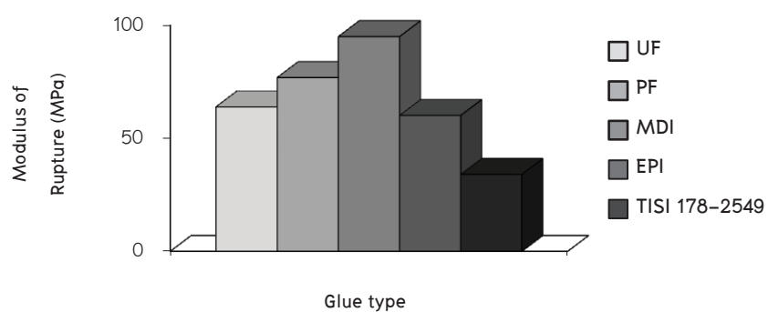
Figure 3. Modulus of rupture of Azadirachta indica .
