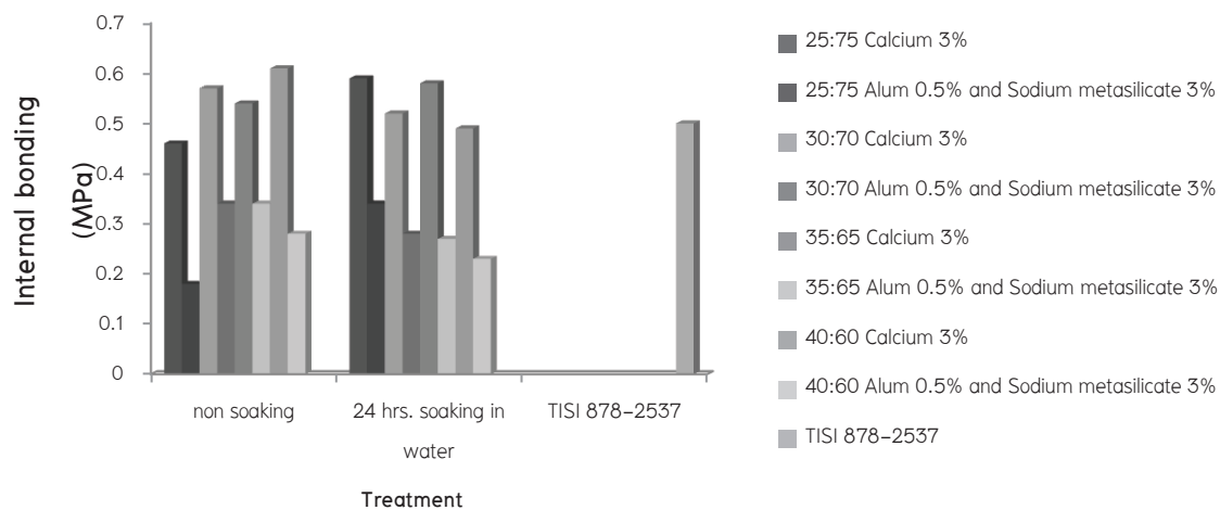
Figure 5. Internal bonding of wood cement boards from Azadirachta indica A. Juss.
