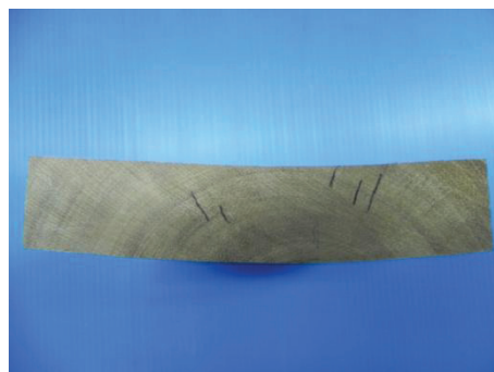
Figure 7. Measuring honeycombing.
