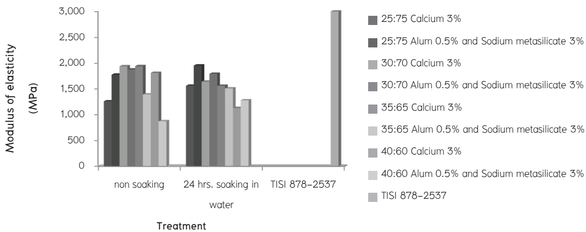
Figure 4. Modulus of elasticity of wood cement boards from Azadirachta indica A. Juss.
